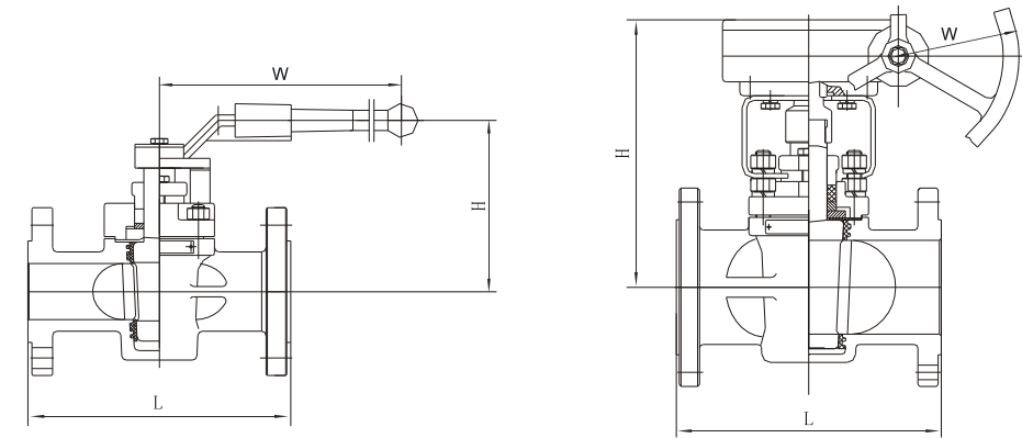
Sleeve type soft sealing plug valve
