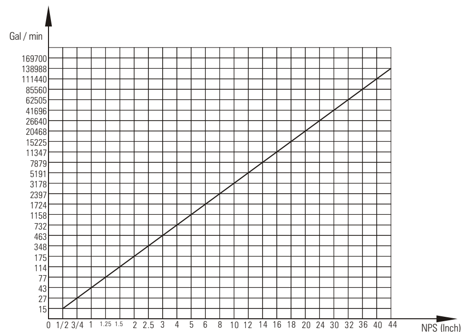
Plug valve torque value list
